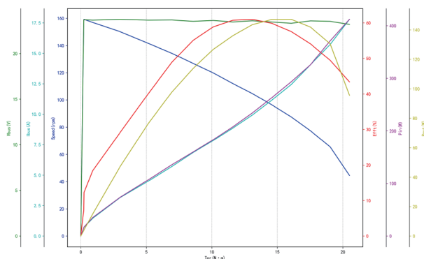
Motor dm216 Performance Curve At 24V
