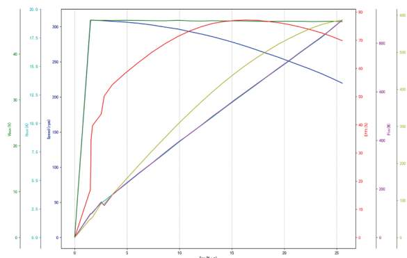
Motor Performance Curve At 48V
